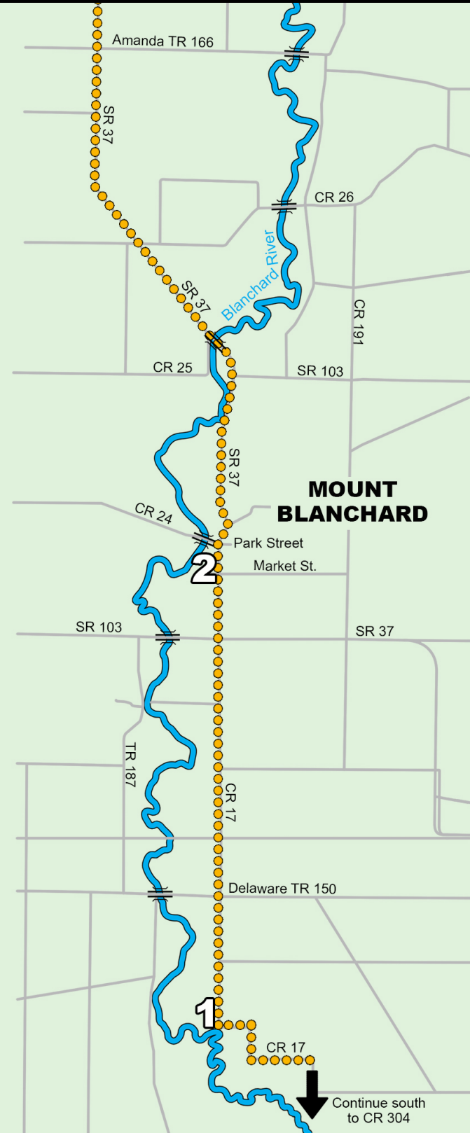
Gilboa Quarry
